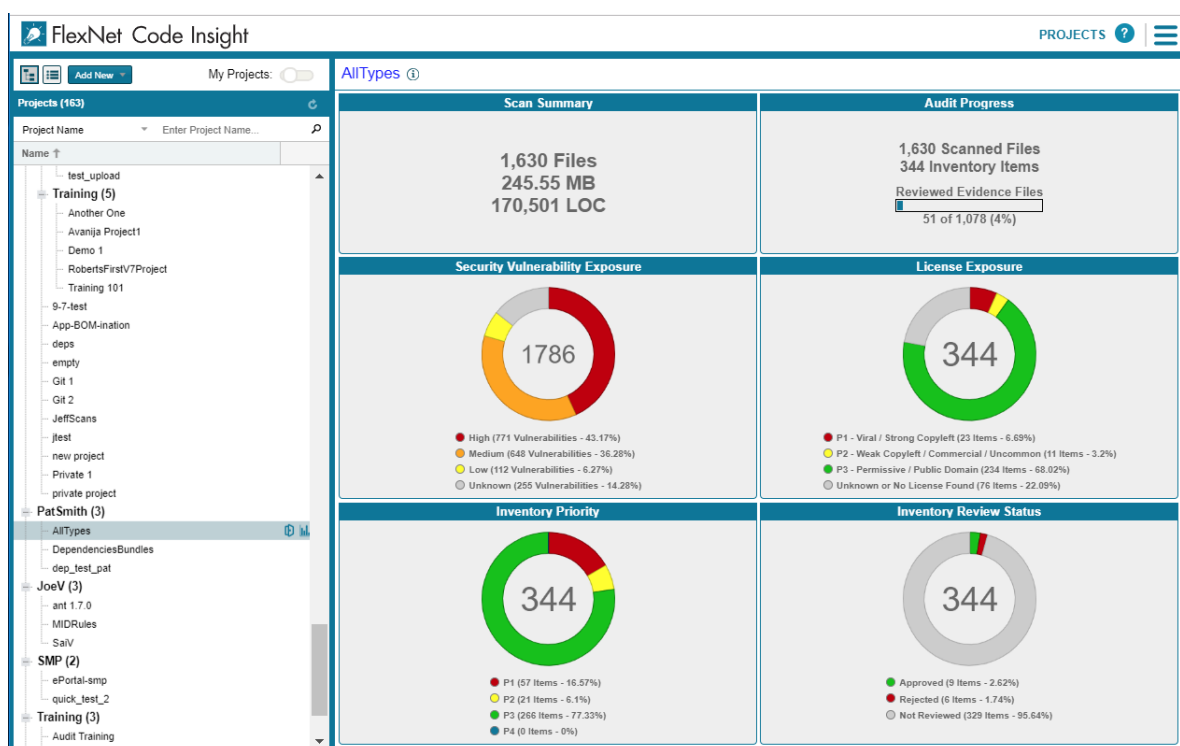
Figure 3: Project Dashboard
