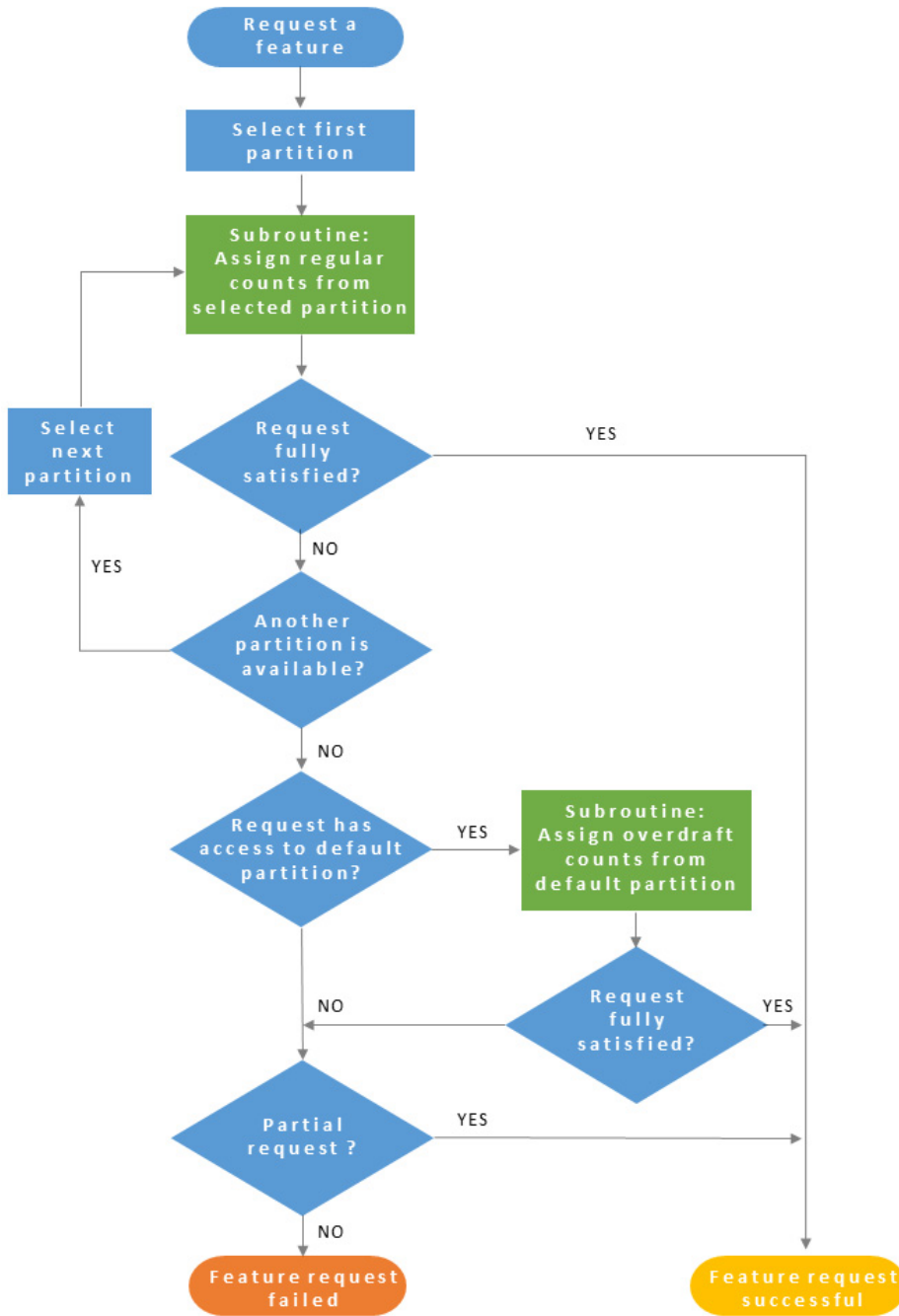
Figure 5-2: Flow of feature allocation
