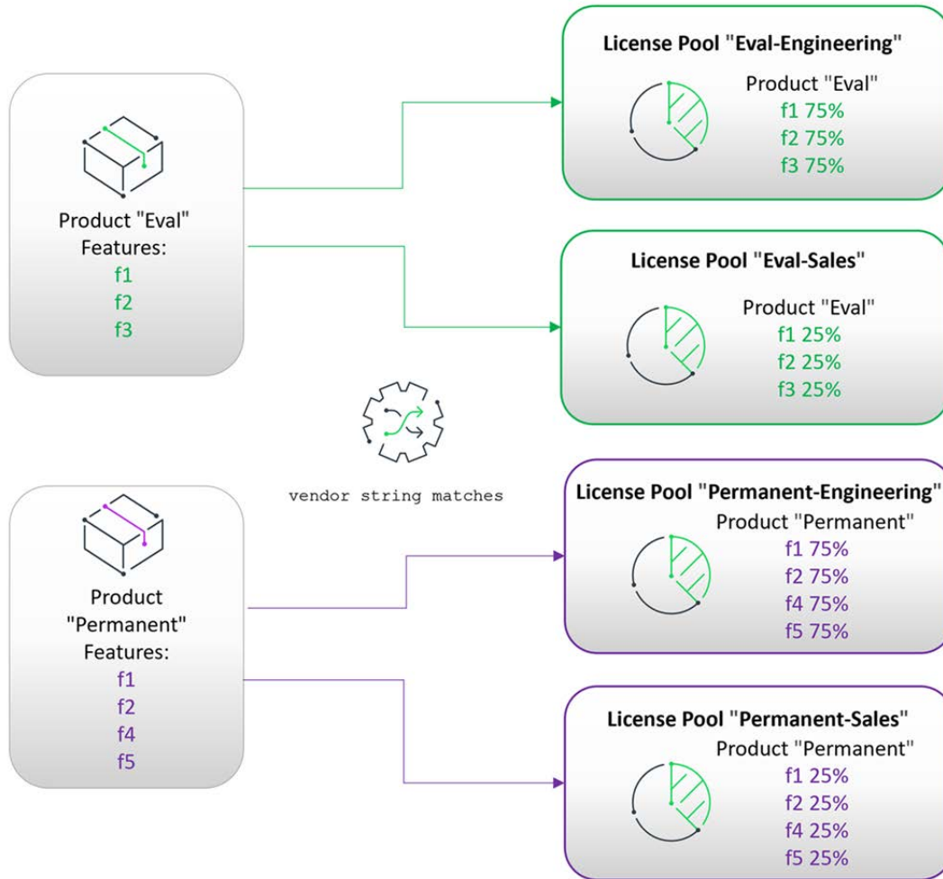
Figure B-1: "vendor string matches" Directive
