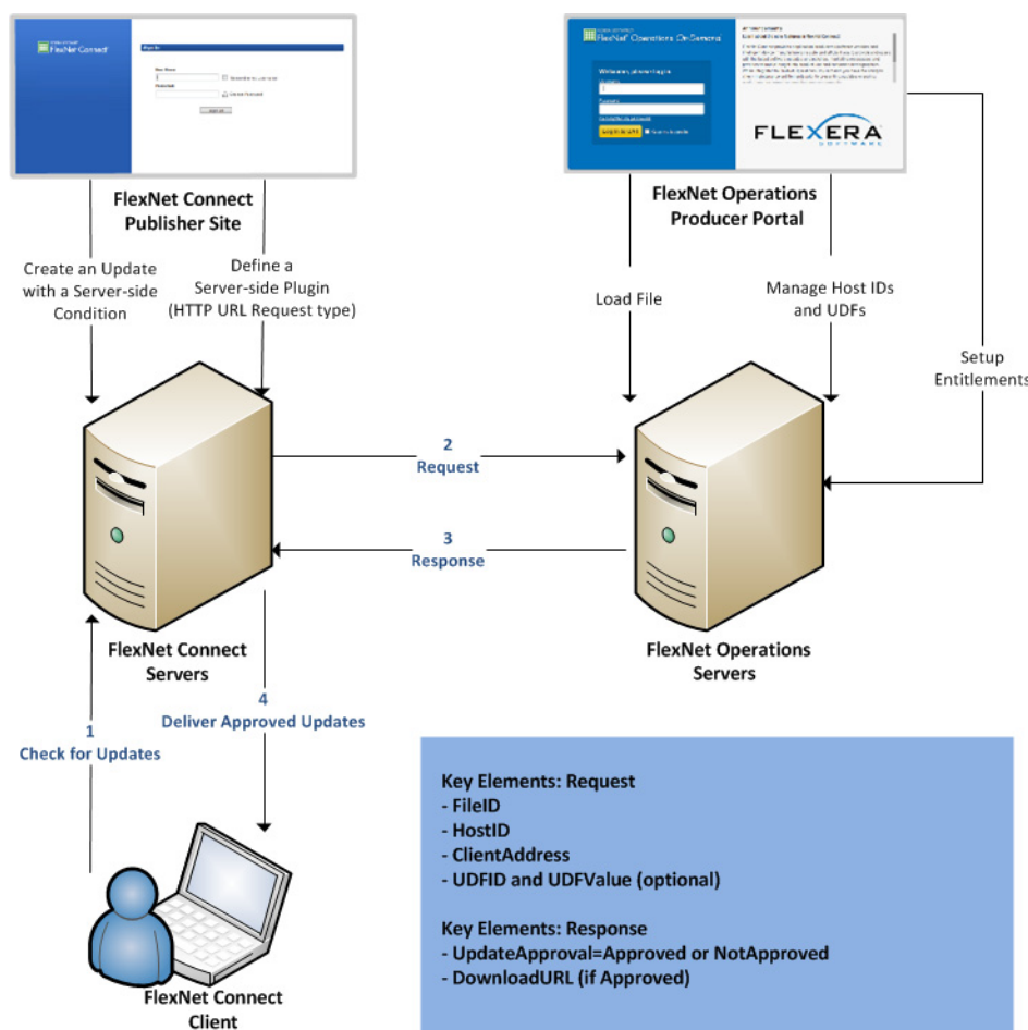
Figure 2-1: Communication flow between FlexNet Connect and FlexNet Operations.
