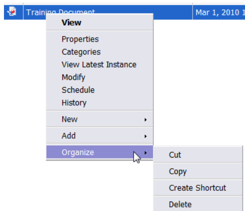
Figure 22-2: Menu options.
