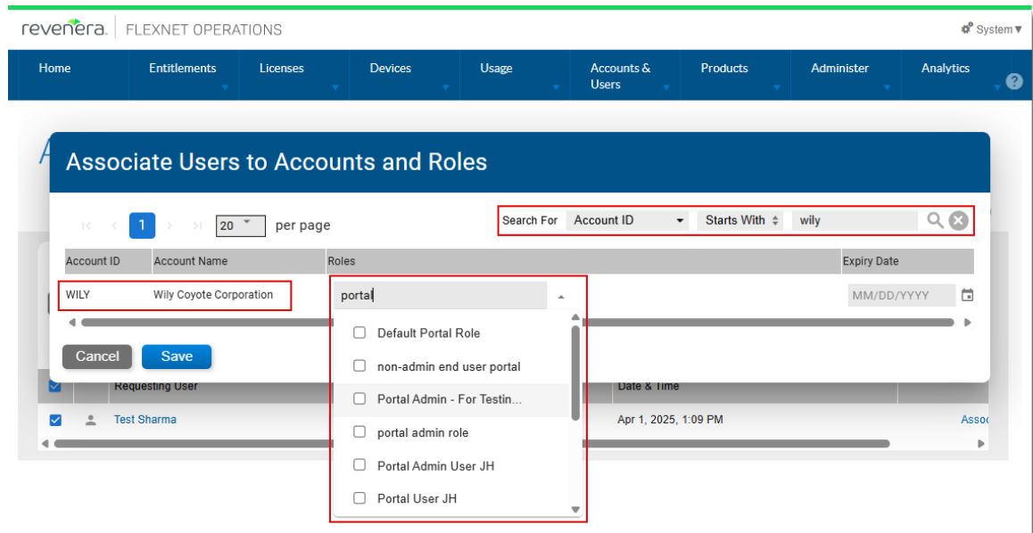
Figure 15: Example view of the Associate Users to Account and Roles window. The search bar is used to locate a specific account, and the Roles field supports text-based filtering to narrow down role selections.
