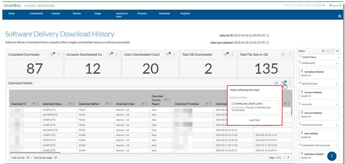
Figure 45: By default, the DOWNLOAD_START_DATE filter is set to show download data for the last 12 months from the current date.
