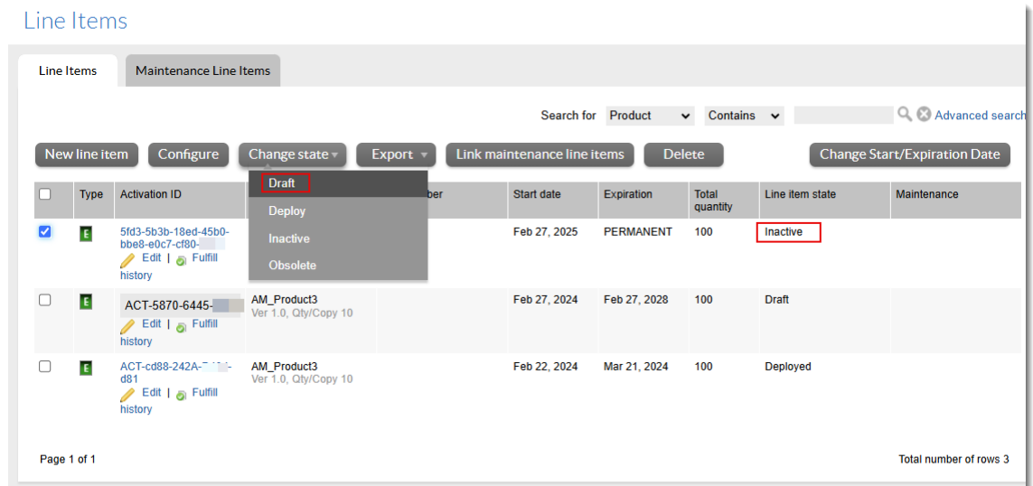
Figure 33: Changing the line item status from Inactive to Draft in the Line Items section of the Entitle Customers to Licenses page
