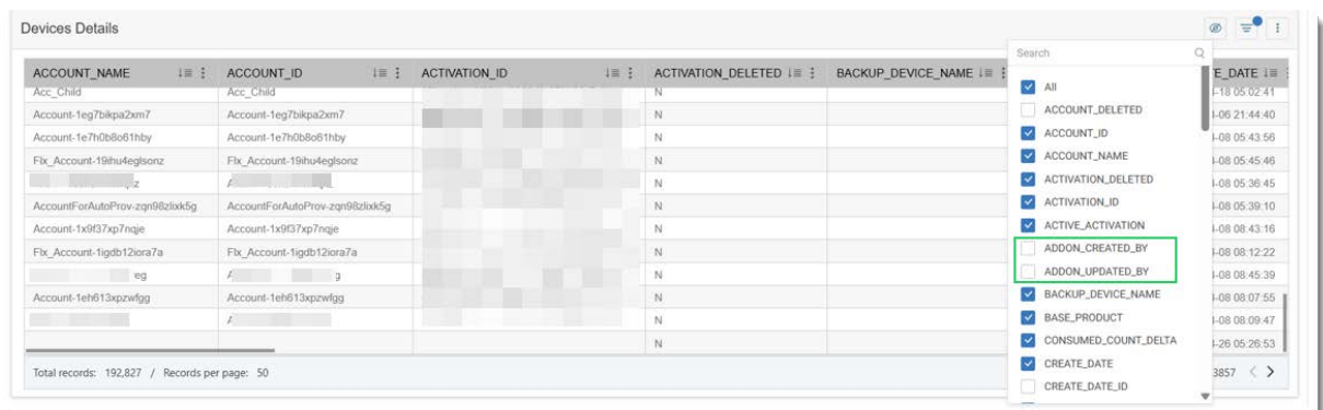
Figure 78: An example view of the Devices Details table in Analytics, with newly added columns being unselected by default.
