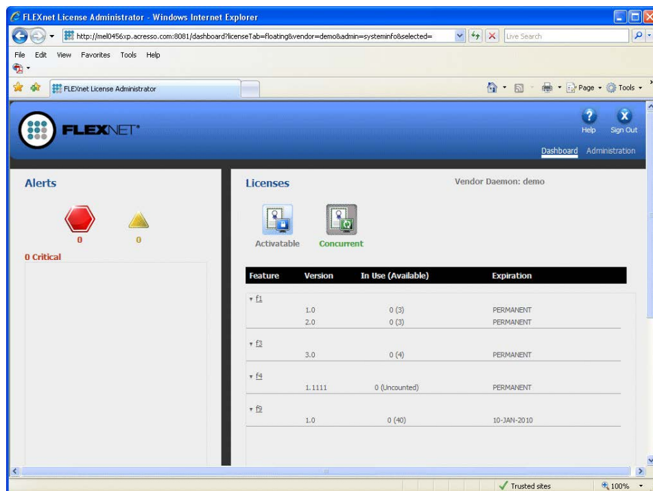
Figure 9-1: lmadmin UI
