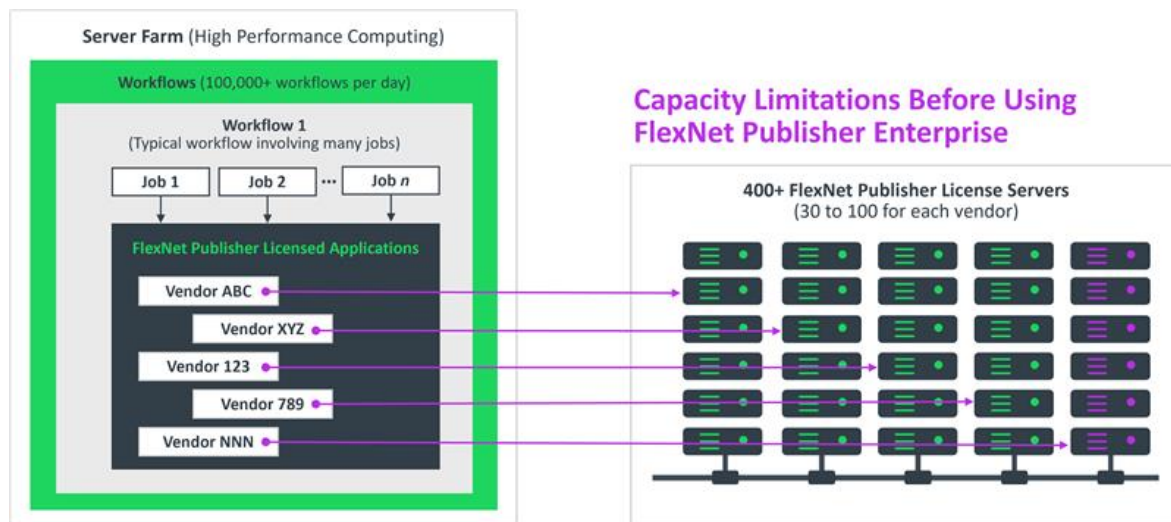
Figure 25-1: License Server Capacity Limitations Before Using FlexNet Publisher Enterprise
