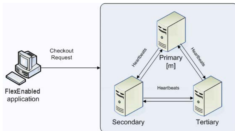
Figure 14-1: Three-Server Redundancy Overview
