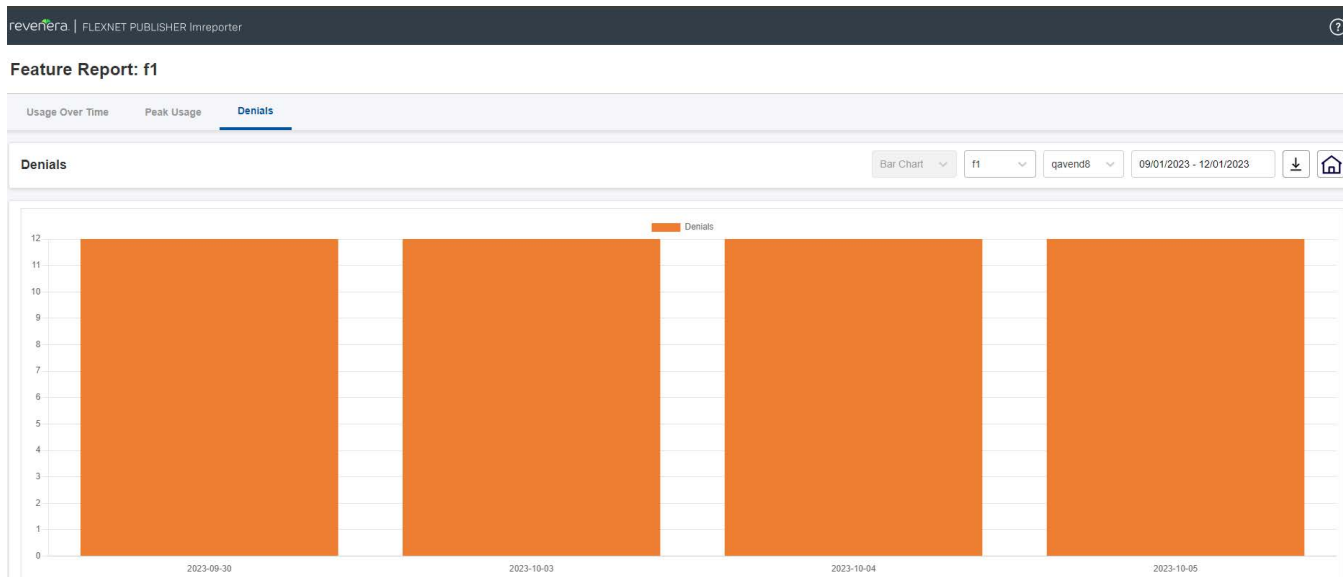
Figure 12-15: Denials Tab
