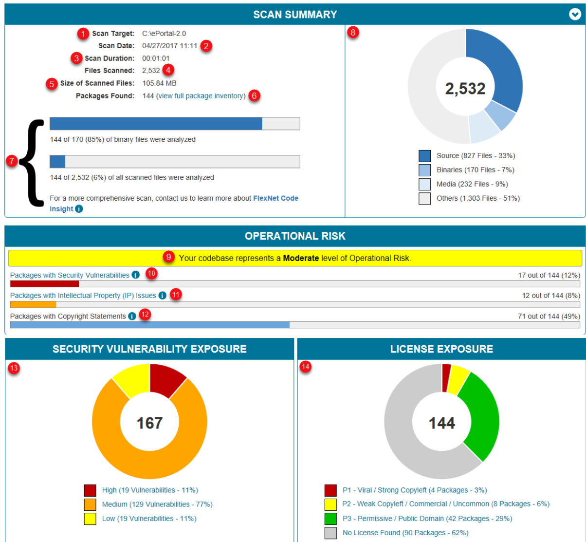
Figure 10-3: Main Areas of the FlexNet Code Aware Report
