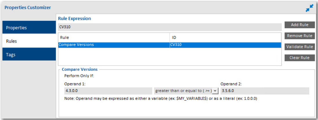
Figure 11-2: Compare Versions Rule Properties Customizer
